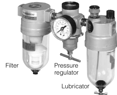
Filter-Regulator-Lubricator assembly (Part No. 173111)
